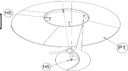
COMPLETE ASSEMBLY
