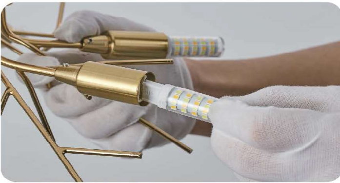
3. Installation of G9 bulbs and available in 5W, 7W, 9W and 12W, depending on your actual needs.
