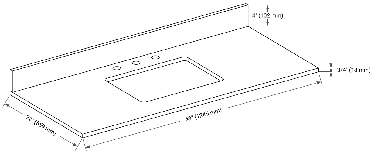
THREE DIMENSIONAL COUNTERTOP VIEW
