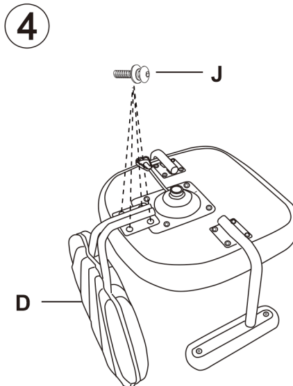
4. Assemble the backrest and the seat cushion together.
