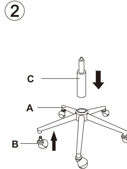
2. Install the casters into the base, then attach the gas lift to the base.
