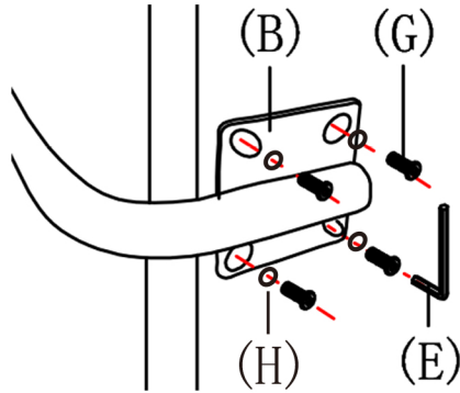
Figure 3: install the tray
