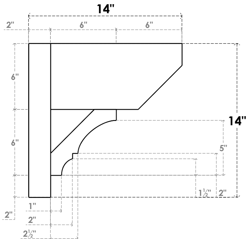
SIDE PROFILE
