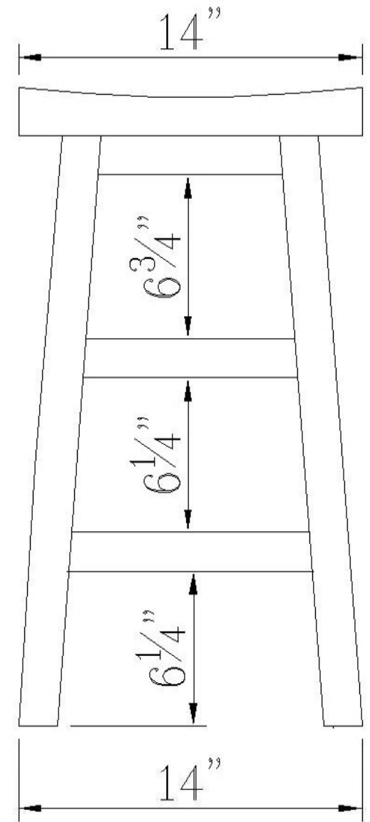
SIDE VIEW
