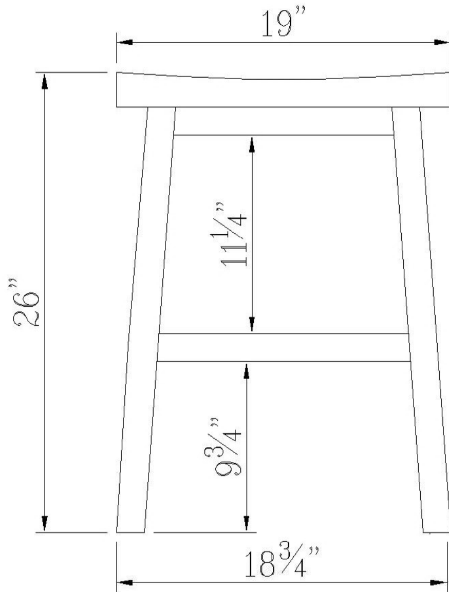
FRONT VIEW
