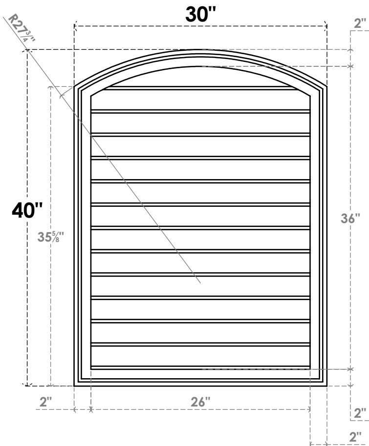
FRONT
