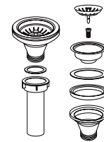
Drain Assembly
