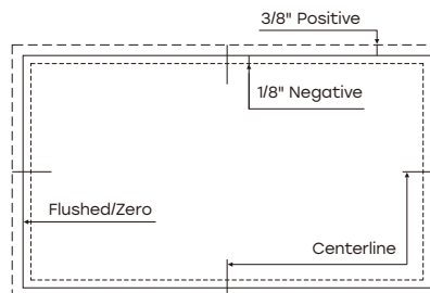
Flushed/Zero Reveal HOROW Recommended Installation Type
