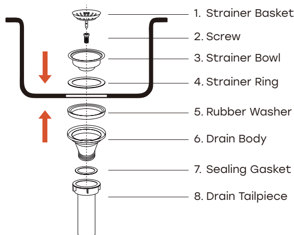
Basket Strainer Assembly Installation
