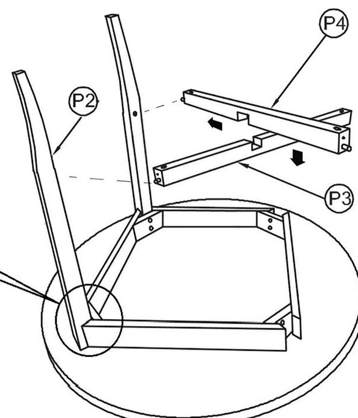
COMPLETE ASSEMBLY
