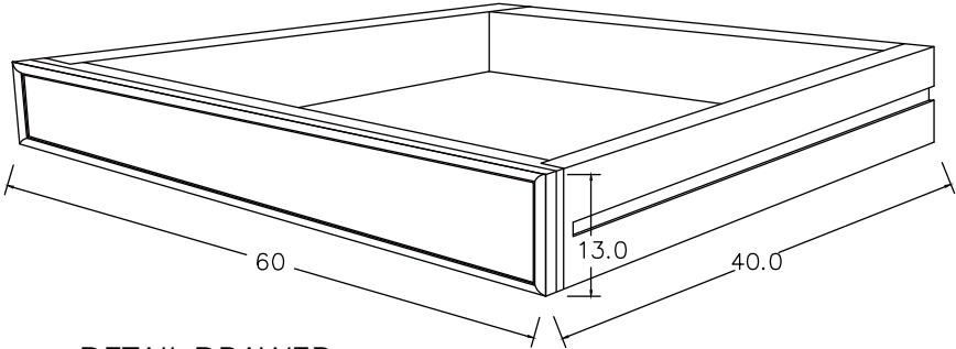
DETAIL DRAWER
