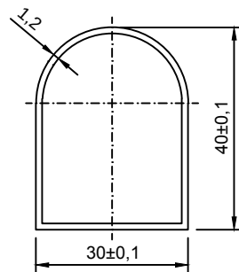
PROFILE DETAIL
