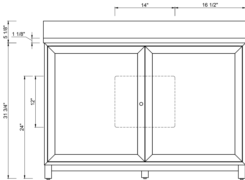
FRONT ELEVATION
