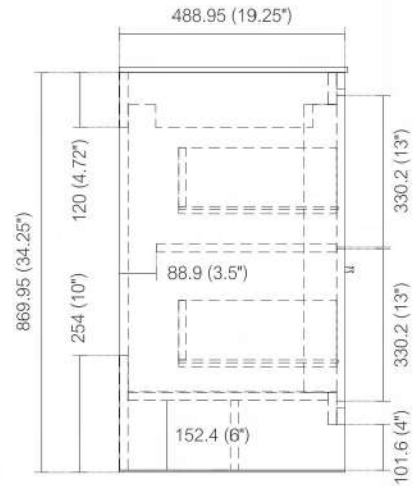
SIDE ELEVATION
