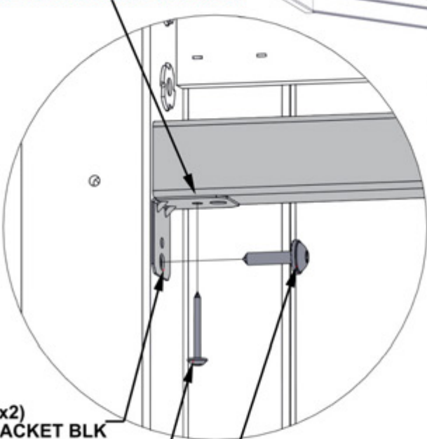
536 (x2) SCREW - 1 1/4"
