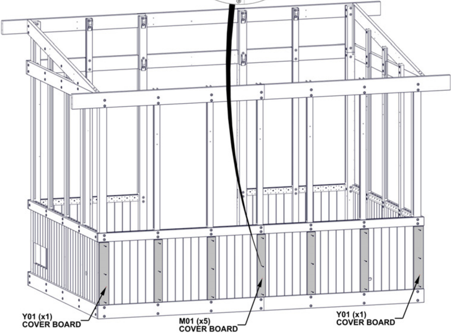
200 (x21) SCREW - 1 1/2"
