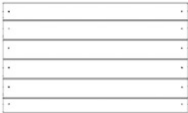
WP03 WALL PANEL - W2A04346 (x3) 1 1/16"x18 7/8"x31 9/16" (27x480x801)
