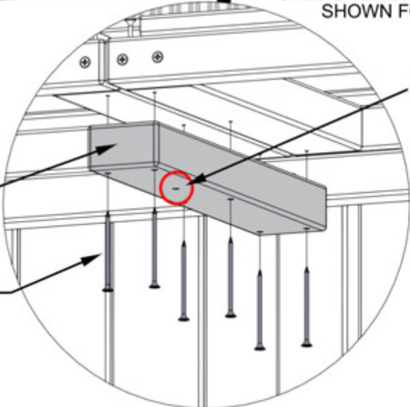
ENSURE PILOT HOLE IS ORIENTED TO THE FRONT AS SHOWN.
