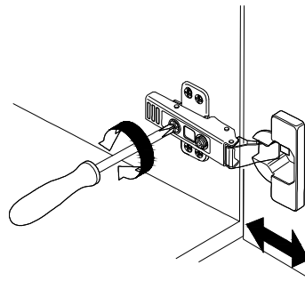
Adjust depth
