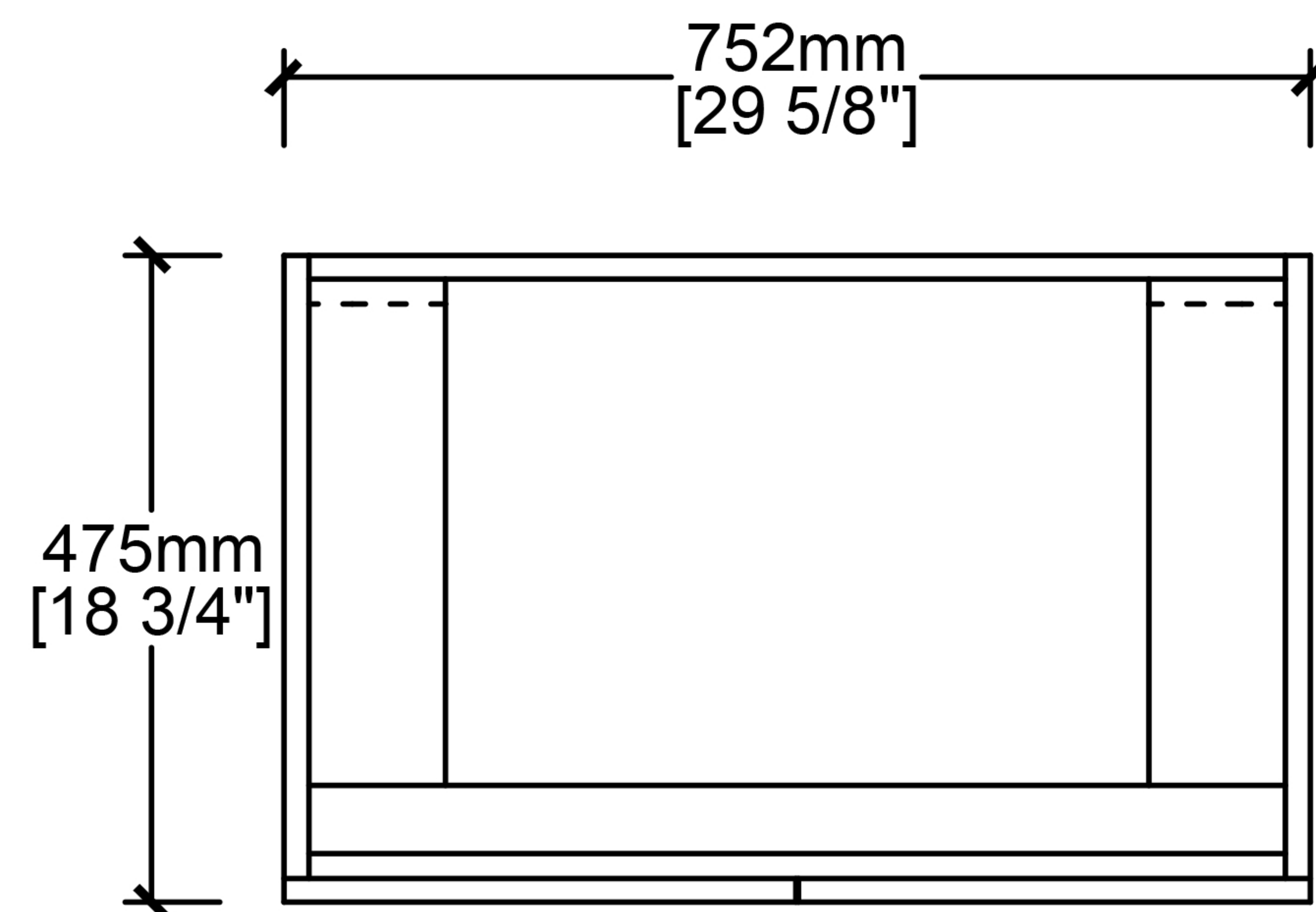
Top view
