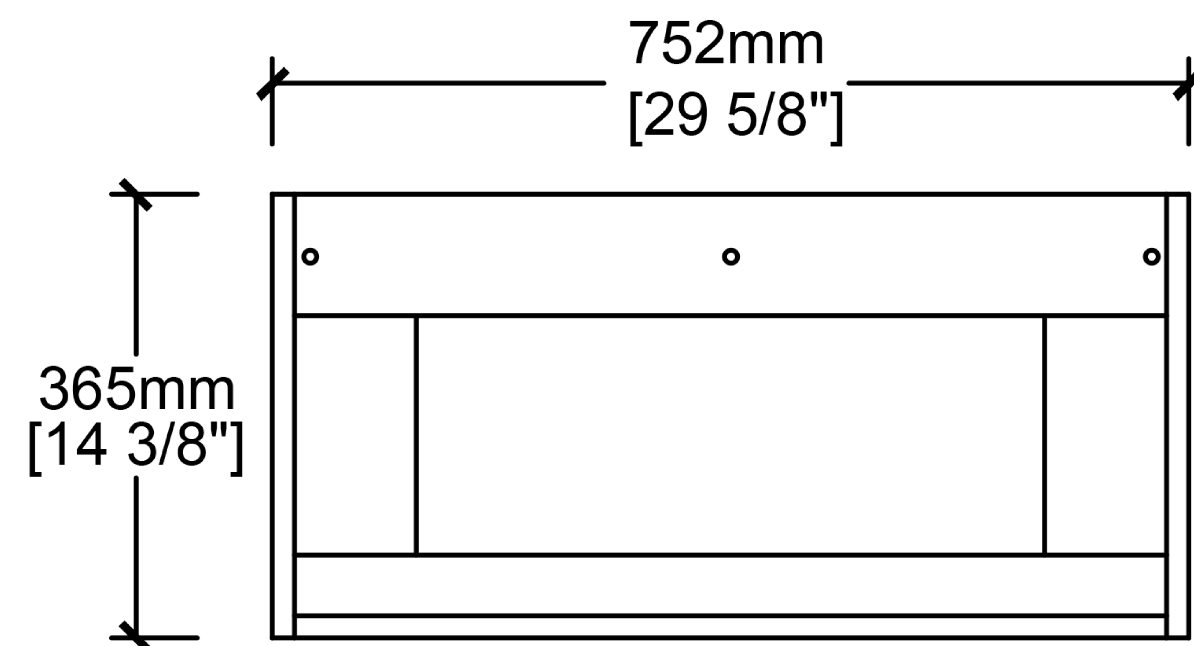
Rear View
