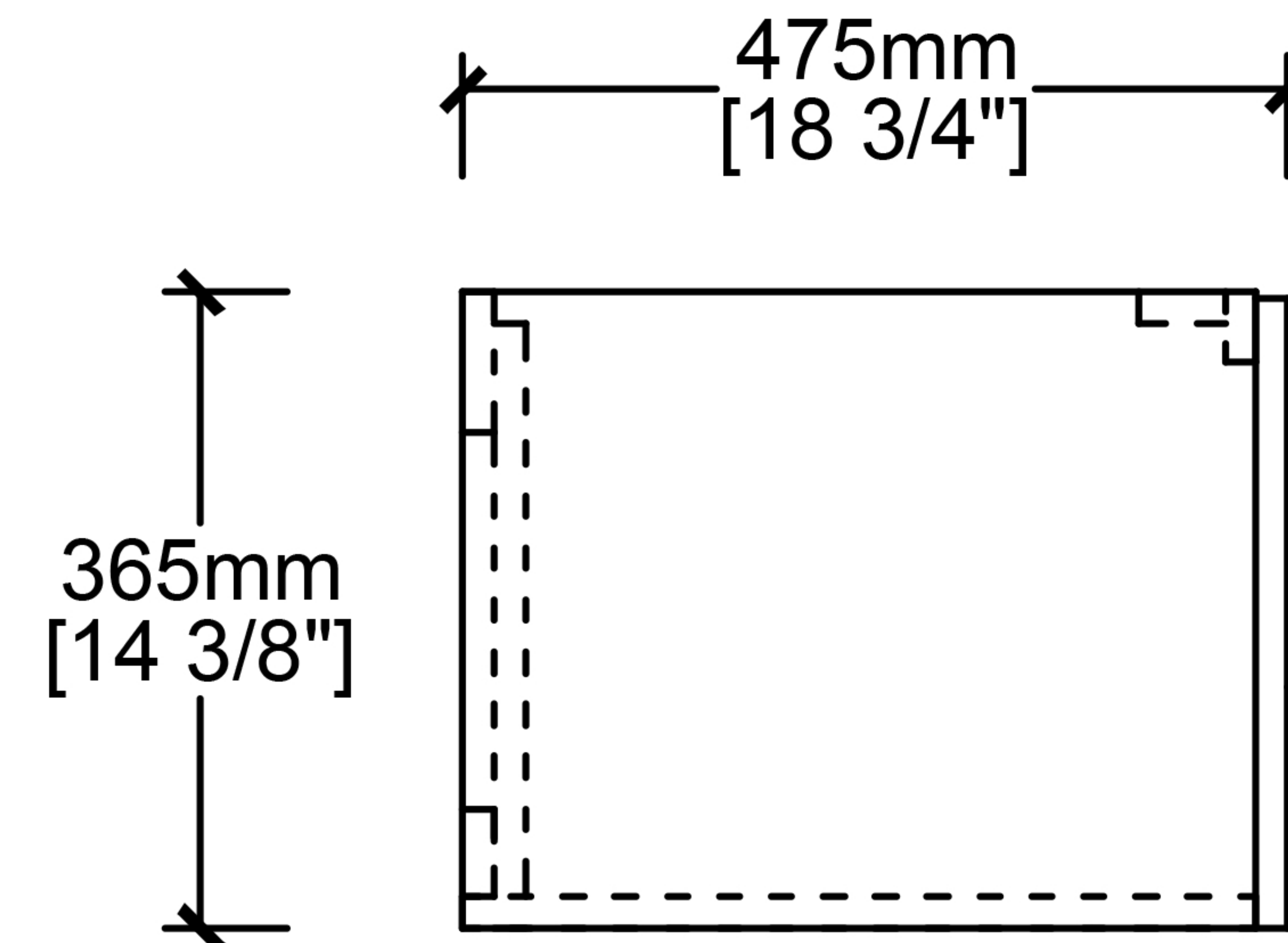
Side View
