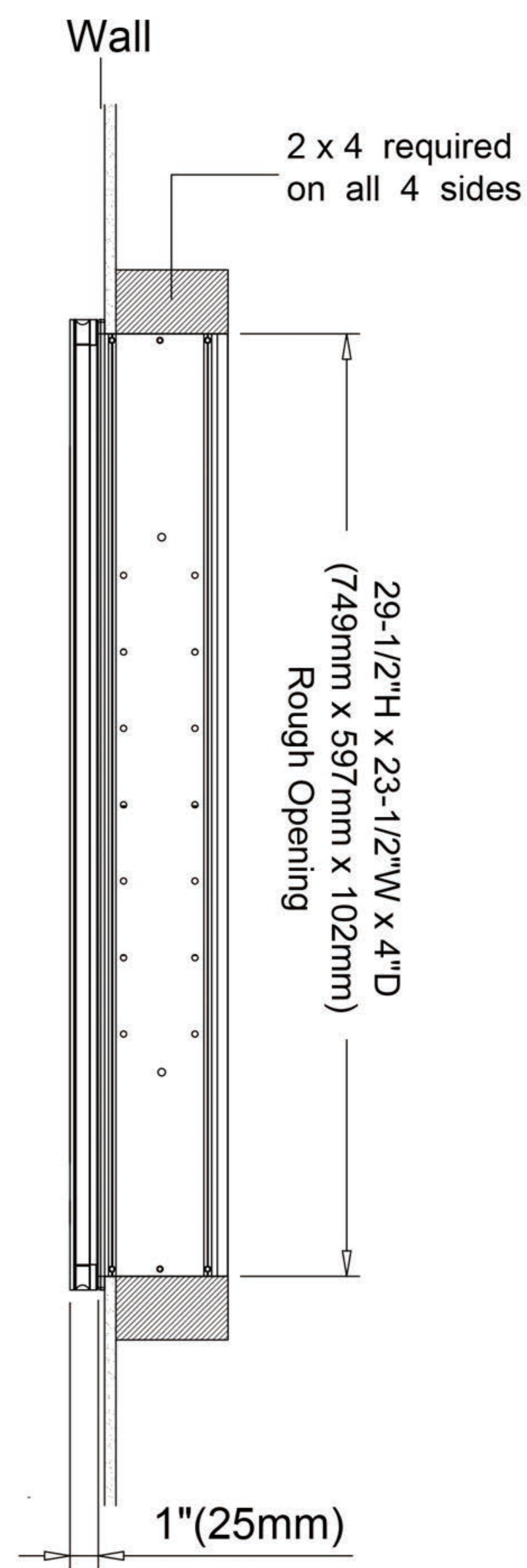
Recessed Mount
