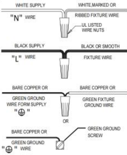
Step 5:Wiring
