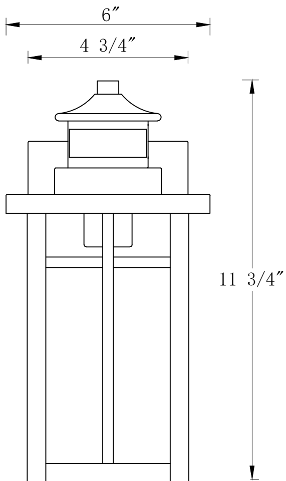
FRONT VIEW
