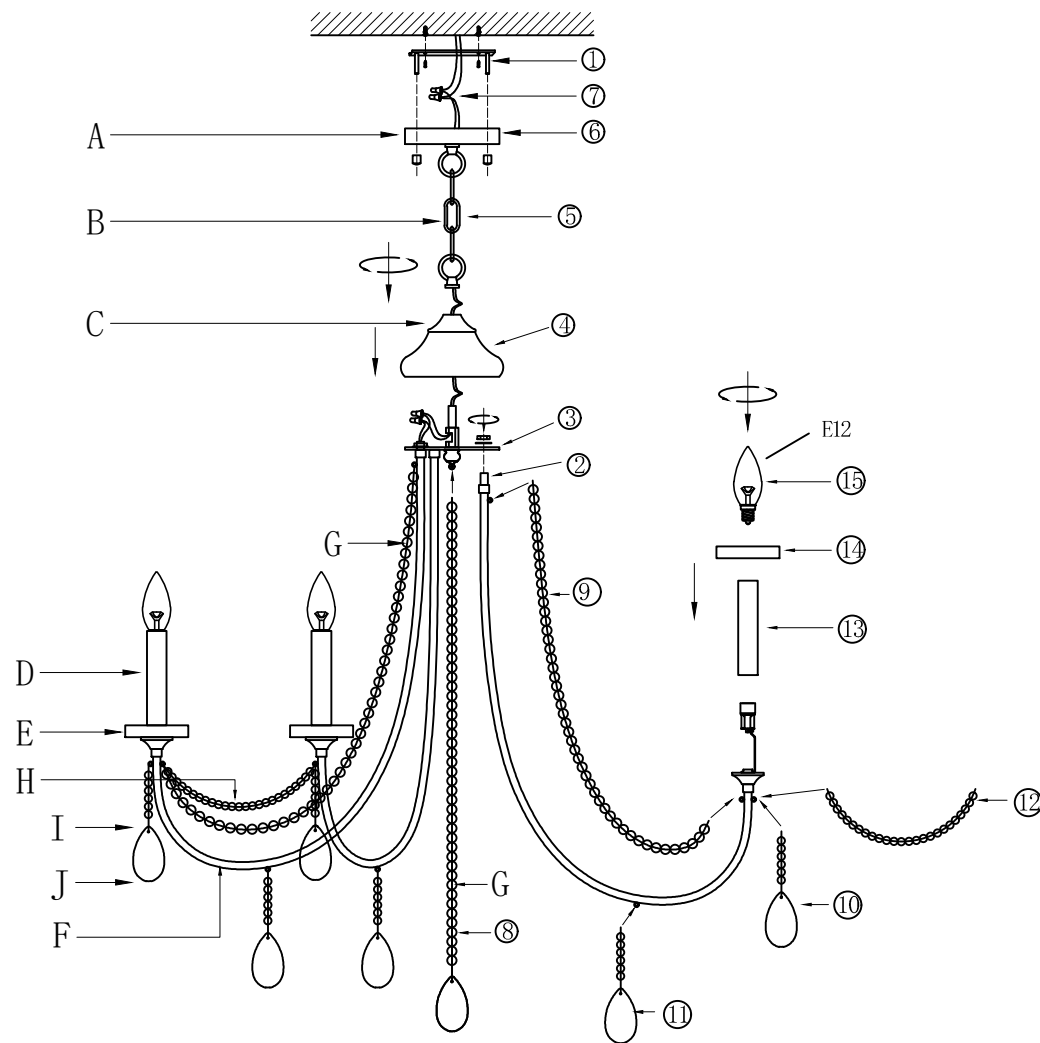
Installation sequence diagram
