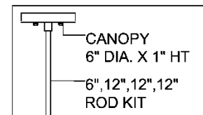
CANOPY DETAIL
