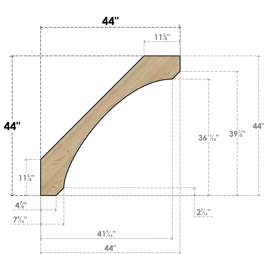
SIDE
