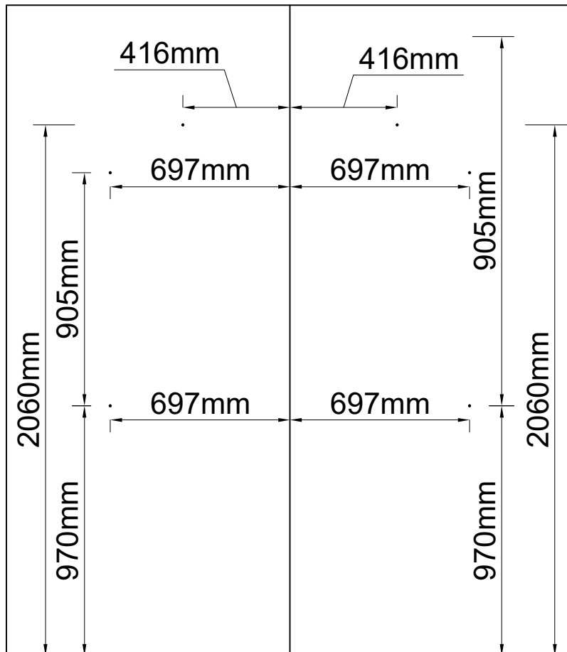
Pre-embedded Hole Location Diagram of the Wall
