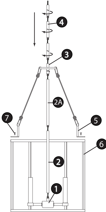
DRAWING 2 - ASSEMBLY
