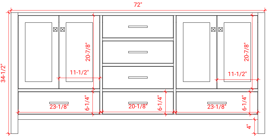
FRONT VIEW
