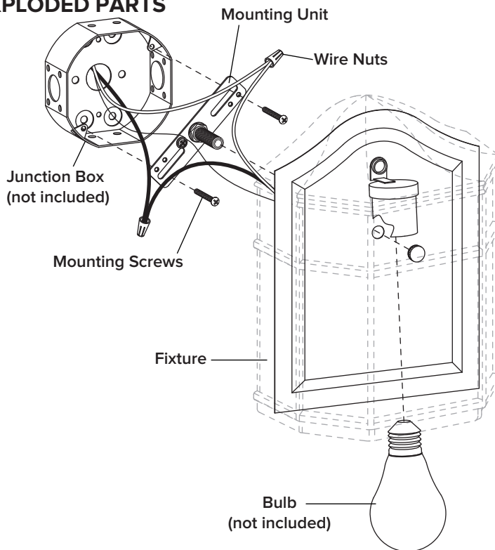
Mounting Unit
