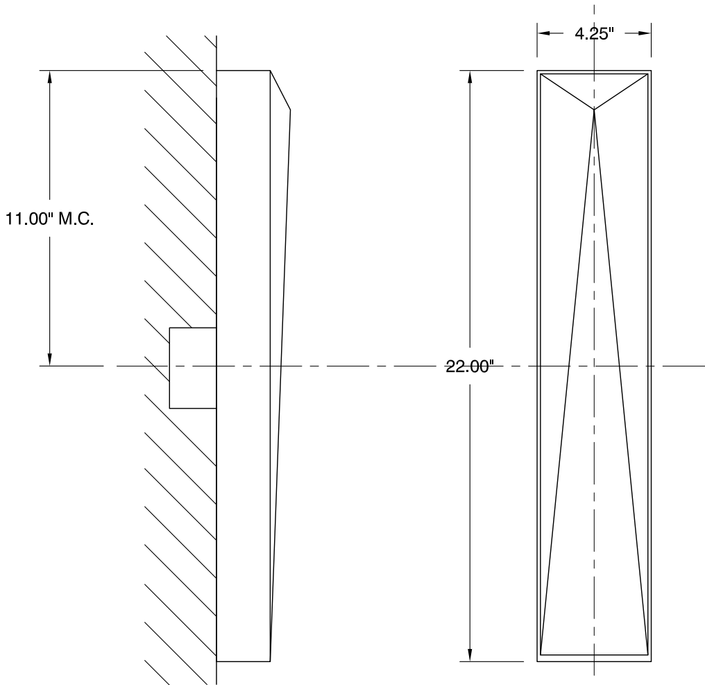
SIDE VIEW
