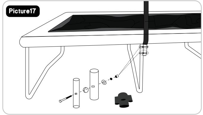
Place the Curved Lower Net Pole with Foam (#11) over the middle leg of the trampoline frame and secure it in place. Firmly Bolt Set (#12) the Lower Net Pole (#11) to the hole of the trampoline 42mm L-shaped Leg (#6-1). Use Spanner (#17) and Allen Wrench (#20) to tighten the Bolts Set (#12).
