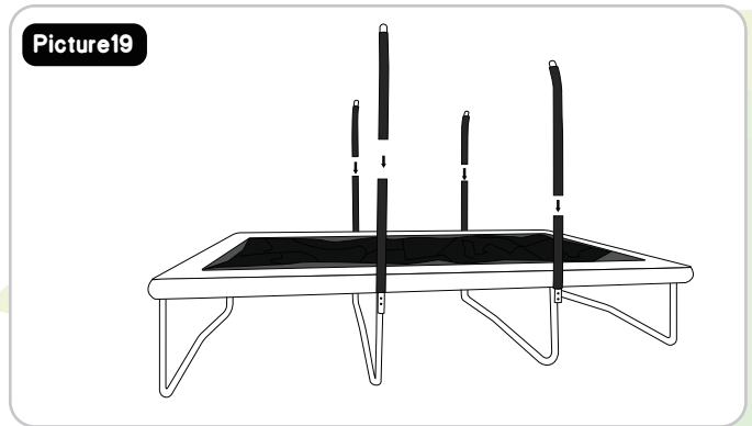
Install the Picture #16 assembled upper net pole (#8) to the lower net pole (#11) as shown. (Note that the groove corresponding to the upper rod faces the inside of the trampoline).
