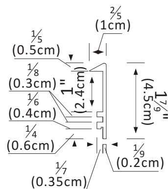
Aluminum section
