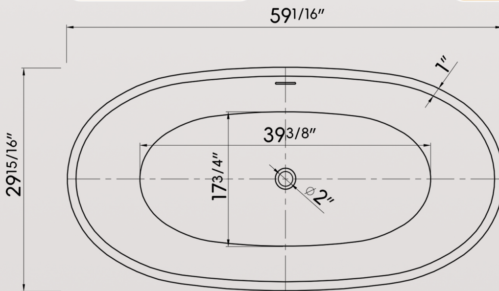
TOP VIEW
