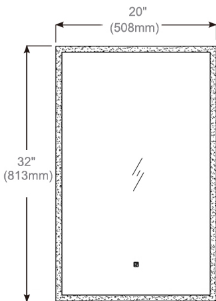
Cabinet Dimensions
