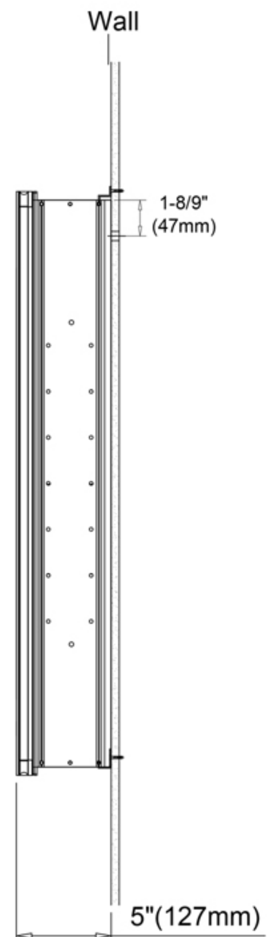
Surface Mount
