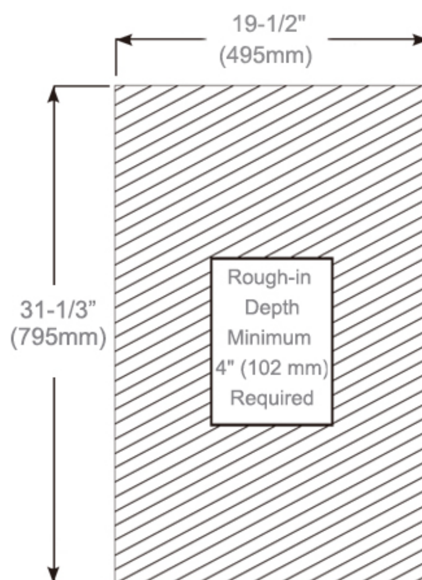
Rough-in Dimensions
