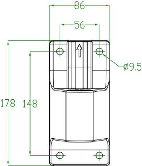
Hole for Plastic Wall Bracket
