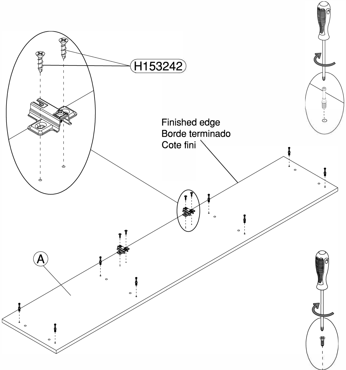
#8 x 5/8"
