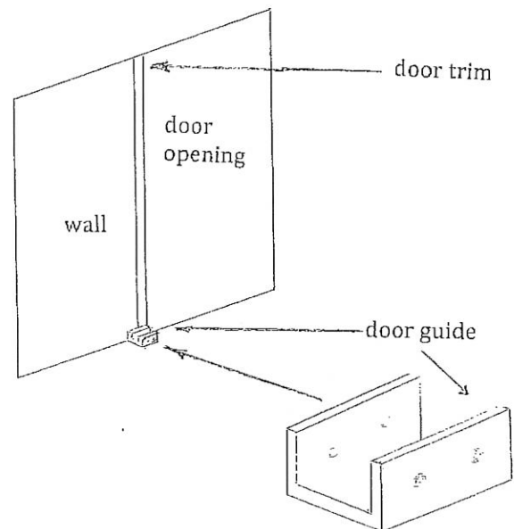
DOOR GUIDE INSTALLATION sliding door and other wall details have been removed to show more detail.
