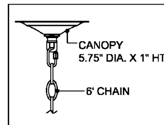
CANOPY DETAIL
