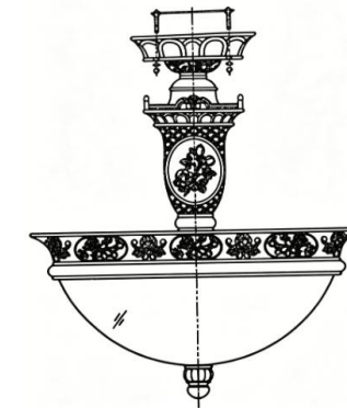
Direct ceiling mounting method
