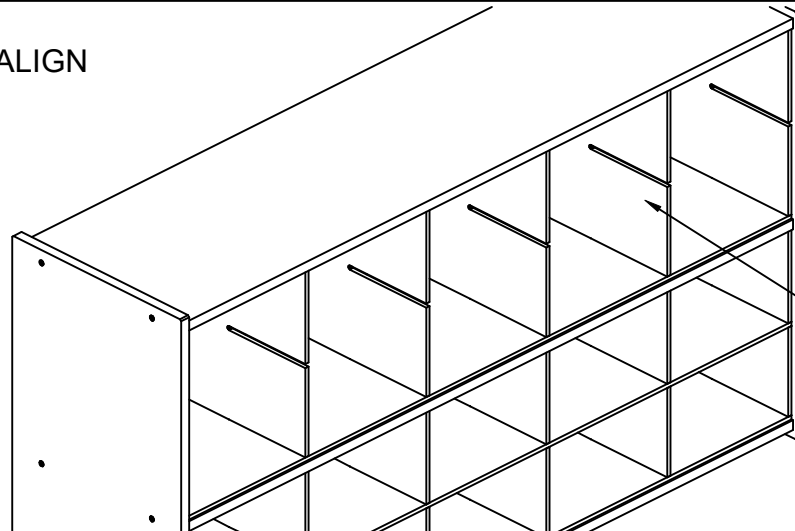
DIVIDER (#508237 - 6 pcs.)
