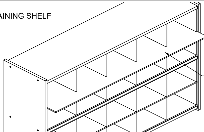
SHELF PANEL (#508236 - 1 pc.)
