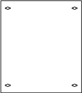
Back
