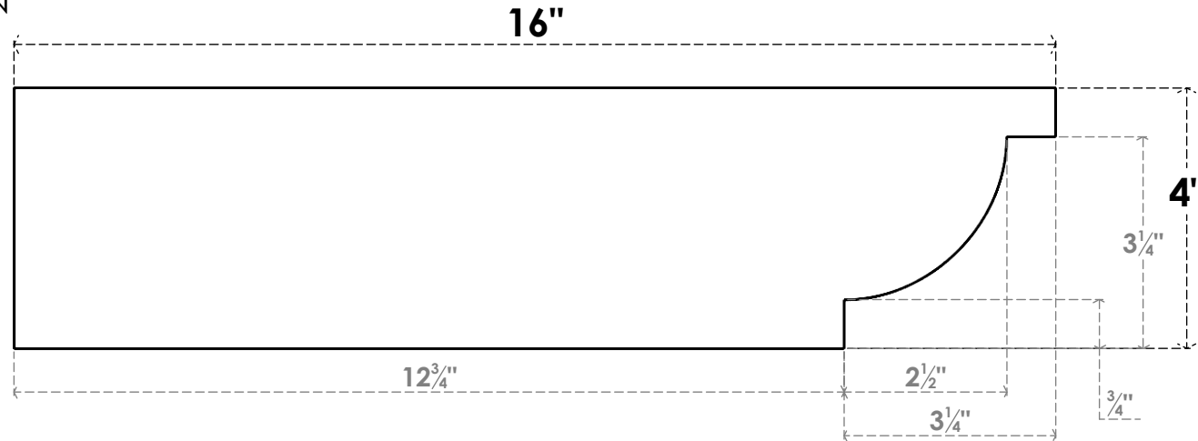
SIDE PROFILE
