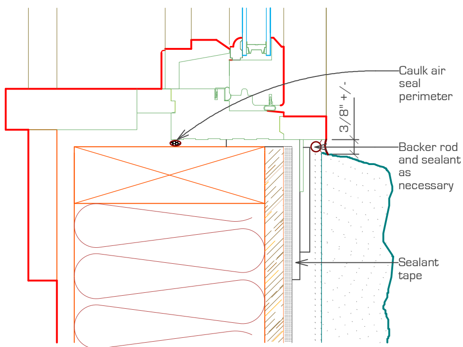
DETAIL # 10
