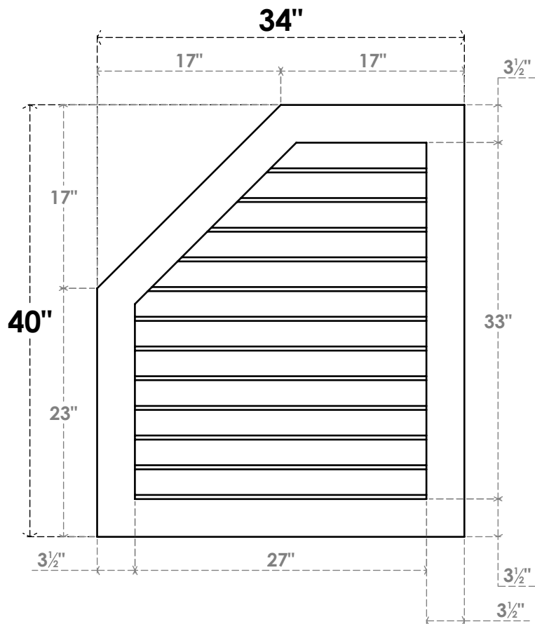
FRONT
