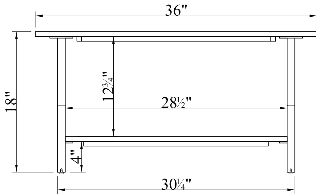
FRONT VIEW
