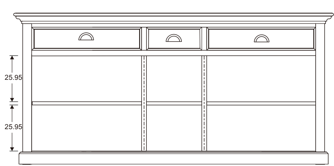
FRONT OPEN VIEW
