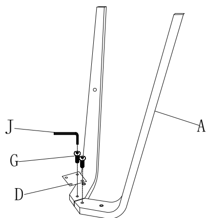
Tighten the screws to 70% tightness. STEP 1
