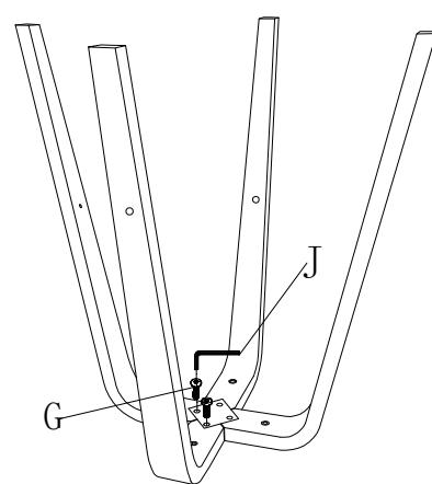
Tighten the screws to 70% tightness. STEP 2
