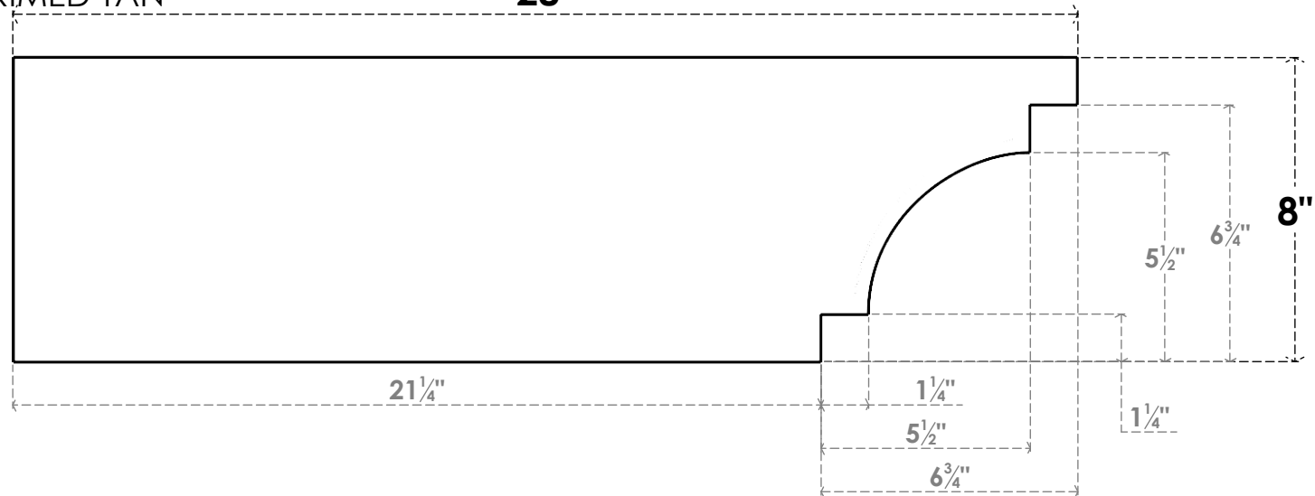
SIDE PROFILE
