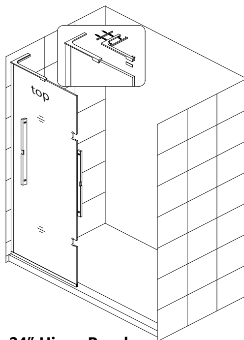
24" Hinge Panel with left L-bracket (#35)
