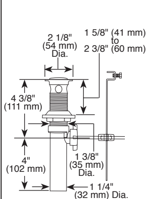
RP38958▲ 50/50 Pop-Up Assembly
