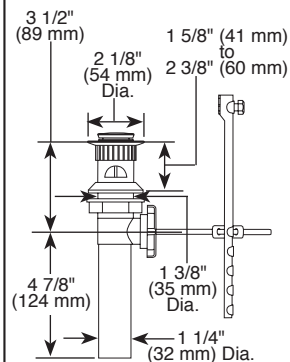
RP34953▲ Plastic Pop-Up Assembly
