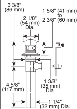
RP26533▲ Metal Pop-Up Assembly
