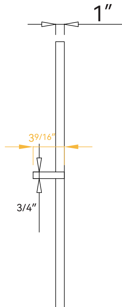
SIDE VIEW
