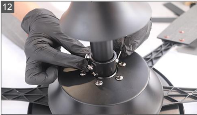
12 Insert the pin removed in Step 6 and secure it with a \beta -shaped needle
