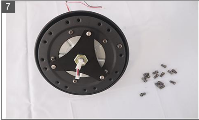
Motor screw removal complete
